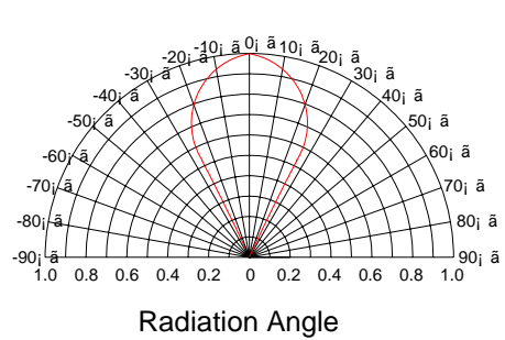
Radiation Characteristics
