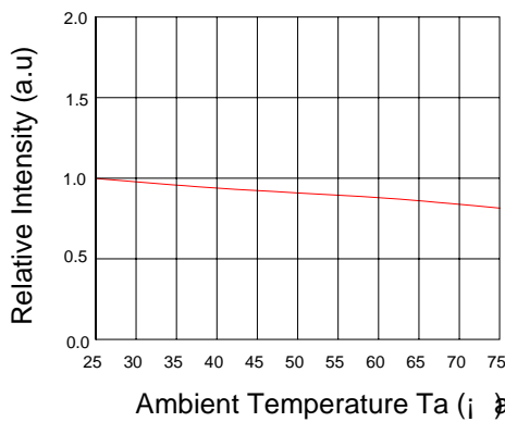
Relative Intensity VS. Ambient Temp
